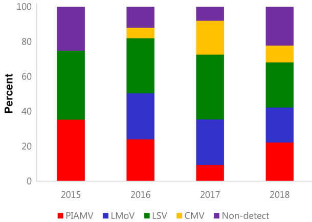
Fig. 1. Occurrence of lily viruses in the fields on Jeju island from 2015 to 2018. PIAMV, Plantago asiatica mosaic virus ; LMoV, Lily mottle virus ; LSV, Lily symptomless virus ; CMV, Cucumber mosaic virus .
