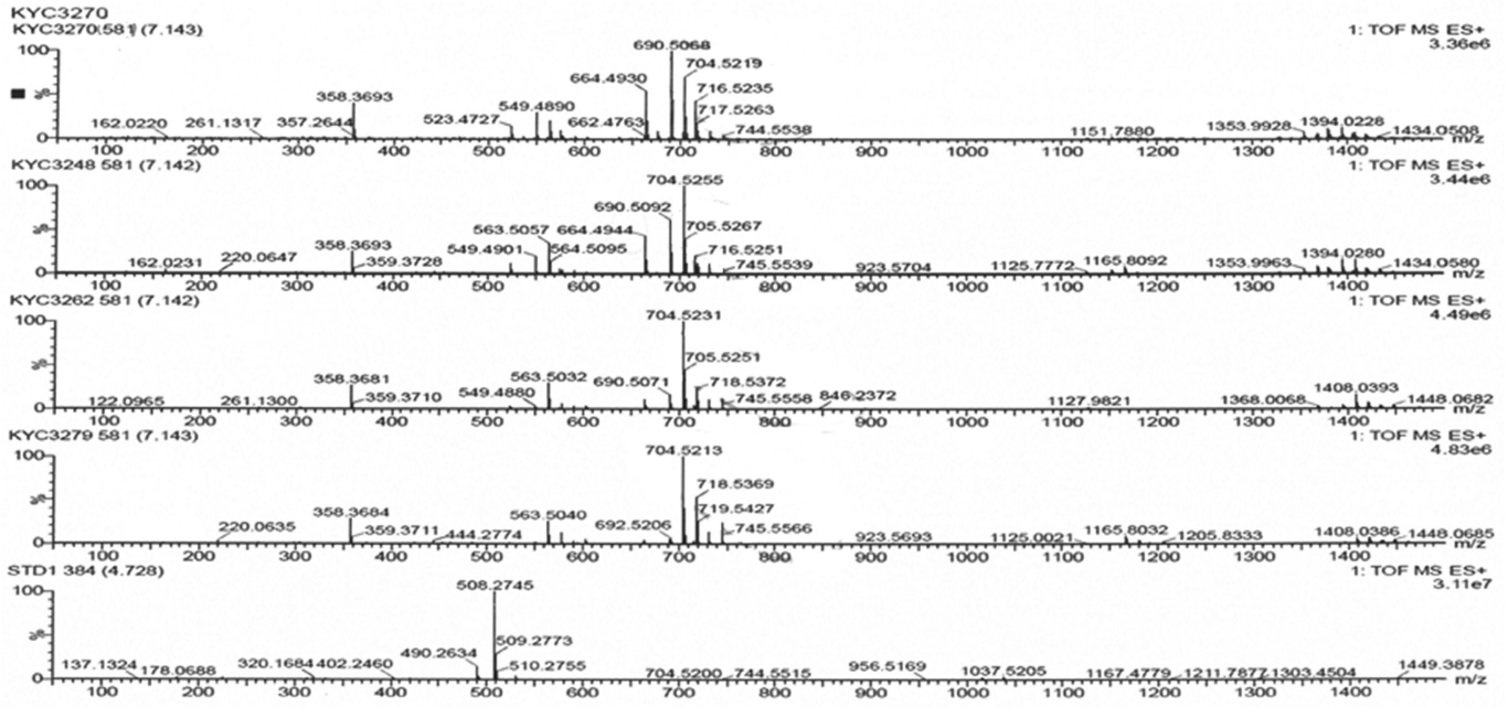
Supplementary data 1. LC-MS chromatograph of KYC 3270 which was known to antagonistic to Botrytis cineria .
